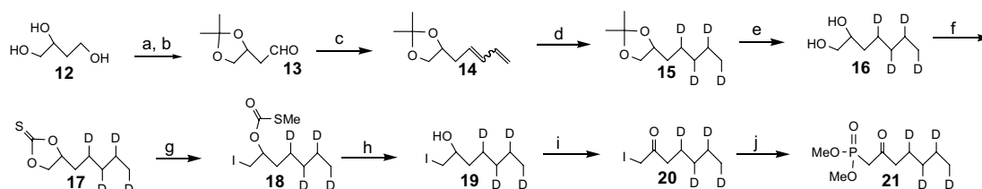
Scheme 3. Reagents and conditions: (a) 2,2-dimethoxypropane, TsOH, CH 3 CN, 1 h, 65%; (b) PCC, camphorsulfonic acid, CH 2 Cl 2 , 3 h, 74%; (c) H 2 C=CHCH 2 P(C 6 H 5 ) 3 Br, LiHMDS, −78 °C to rt, 2 h, 89%; (d) Wilkinson's catalyst, 99.98% D 2 , benzene, 8 h, 87%; (e) 4% H 2 SO 4 , THF, 8 h, 99%; (f) Im 2 CS, CH 3 CN, 94%; (g) CH 3 I, ClCH 2 CH 2 Cl, 70 °C, 10 h, 86%; (h) DIBAL-H, CH 2 Cl 2 , −78 °C, 40 min, 96%; (i) Jones reagent, acetone, 0 °C; (j) P(OMe) 3 , THF, 45 °C, 10 h, 69% (two steps).
