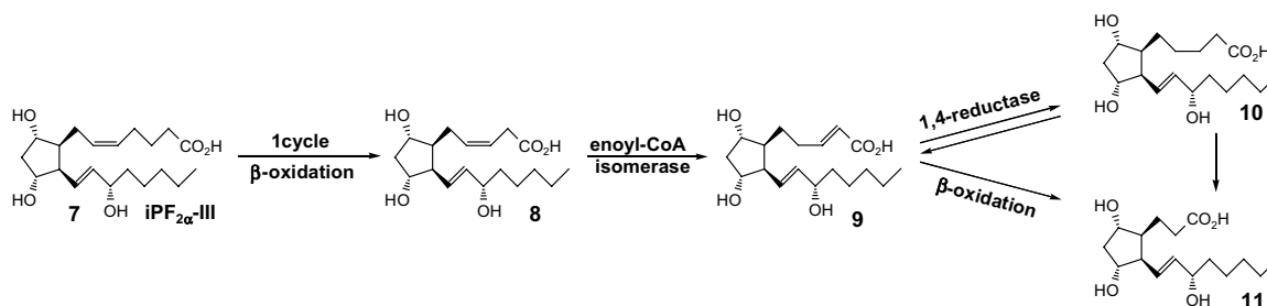
Scheme 2. Proposed metabolism pathway for the formation of 8 , 10 , and 11 .
