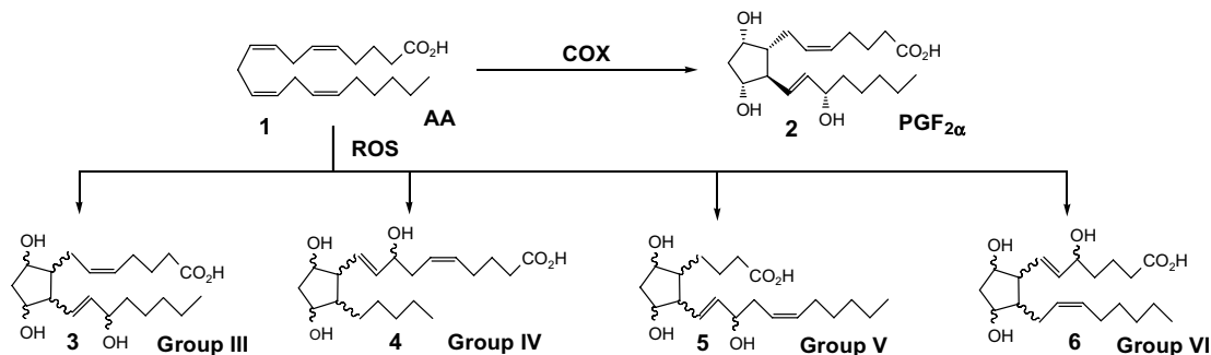
Scheme 1. Groups of isoprostanes derived from AA.
