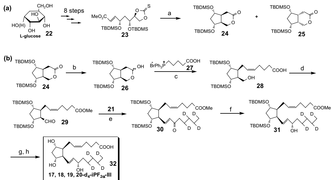
Scheme 4. Reagents and conditions: (a) n -Bu 3 SnH, AIBN, benzene, reflux, 5 h, 52%; (b) DIBAL-H, CH 2 Cl 2 , −78 °C, 87%; (c) t -BuOK, HMPA, THF, −78 °C to rt, 1 h, 68%; (d) periodinane, CH 2 Cl 2 , rt, 8 h; (e) NaHMDS, THF, −78 °C to rt, 72%; (f) ( S )-BINAL-H, THF, −100 °C, 4 h, 99%; (g) THF:formic acid:H 2 O—6:3:1, rt, 8 h; (h) 5% KOH, THF, 0 °C to rt, 3 h, 76% (two steps).
